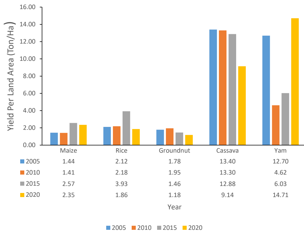
Figure 4. 33 Estimated Yield per Land Area for Benue State
