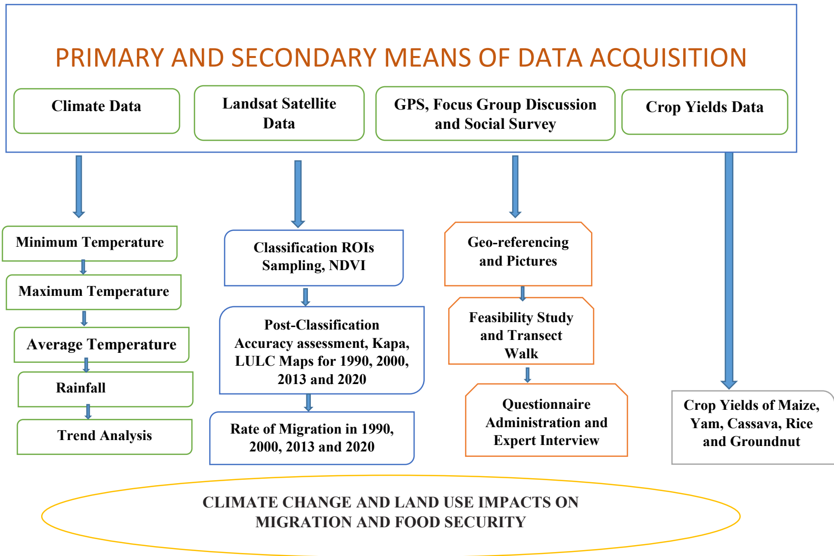
Figure 3. 1 Methodology Flowchart
