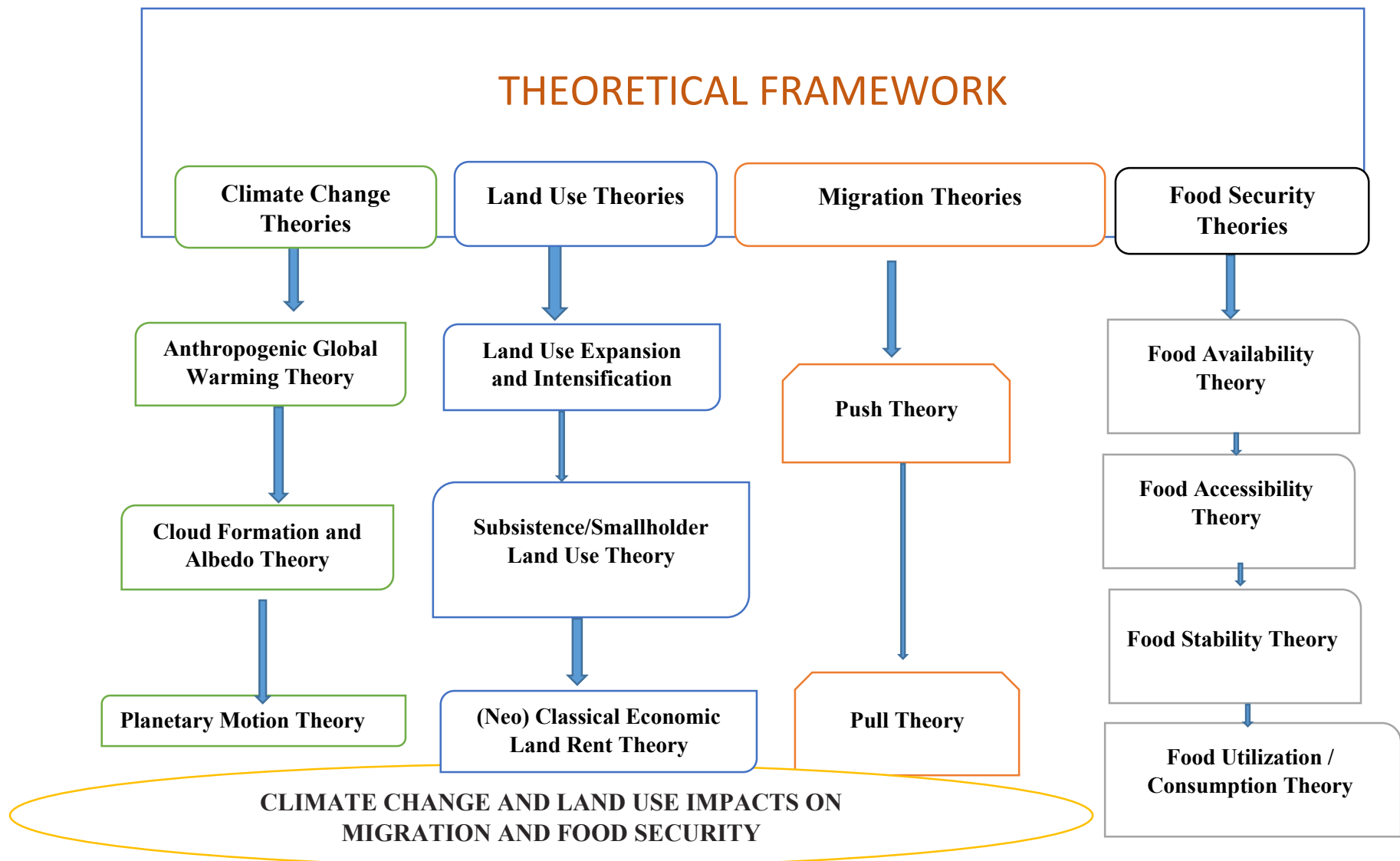
Figure 2.2 Theoretical Framework
